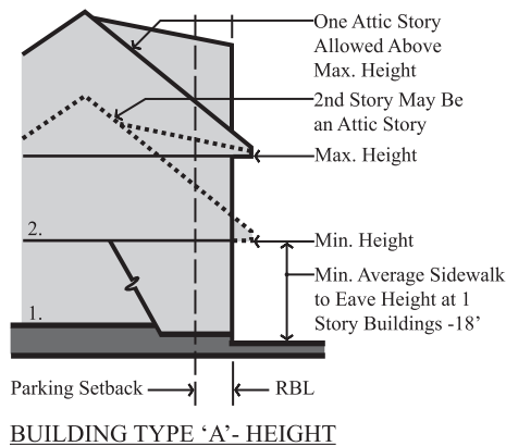
BUILDING TYPE 'A'- HEIGHT
